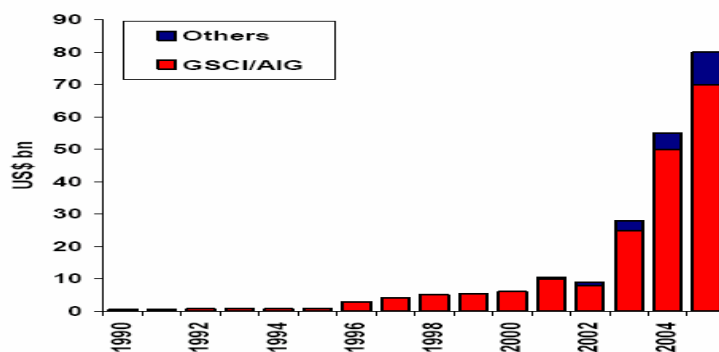
Commodity Index Funds, total investment in US$
